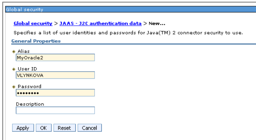
Figure 17: Setting up global security in WebSphere
